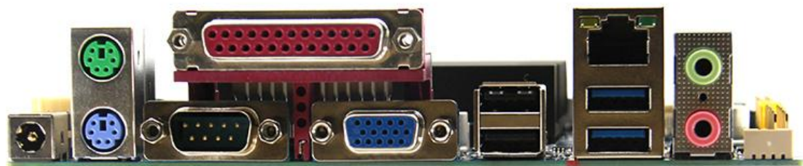
DC_JACK PS/2 COM1 PRINTER VGA USB1 LAN-USB2 AUDIO-JACK
